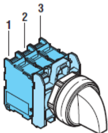
Contact activation of 3-position selector switch
